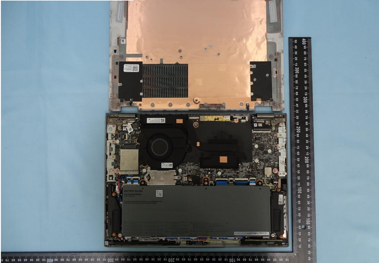
With WLAN Module (AX211D2W)
