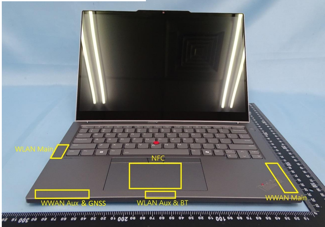
AWAN Antenna and Speed Antenna
