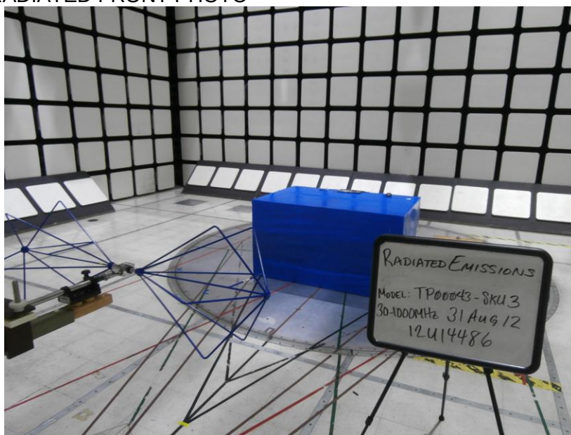
Below 1GHz
