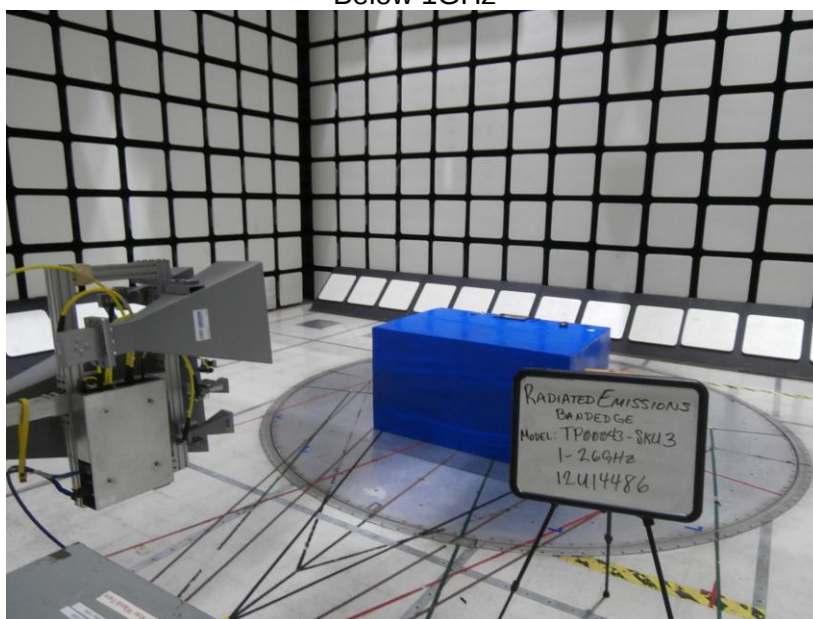
Above 1GHz
