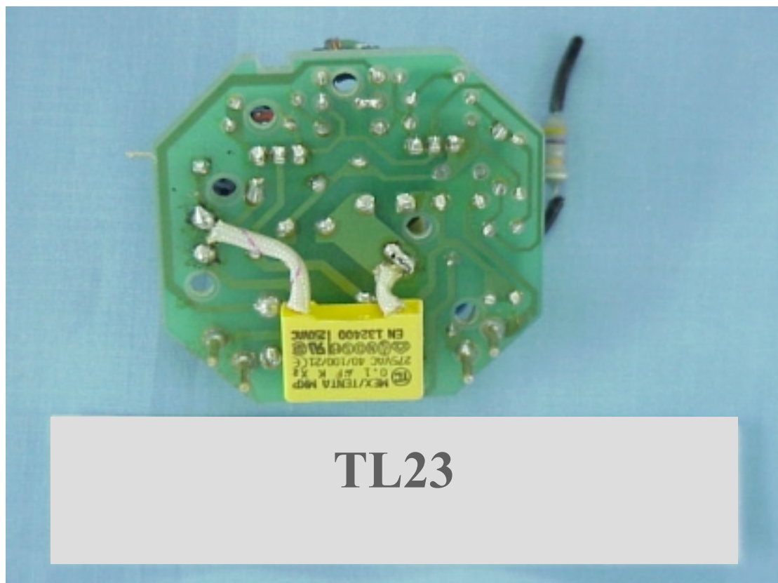
FIGURE 6 TWIST LAMP (M/N: TL23) MAIN BOARD (SOLDERED SIDE)
