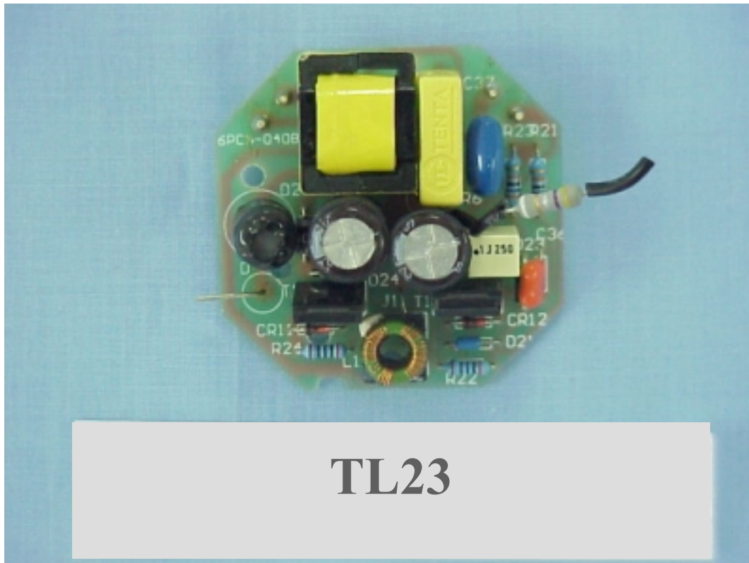
FIGURE 5 TWIST LAMP (M/N: TL23) MAIN BOARD (COMPONENT SIDE)
