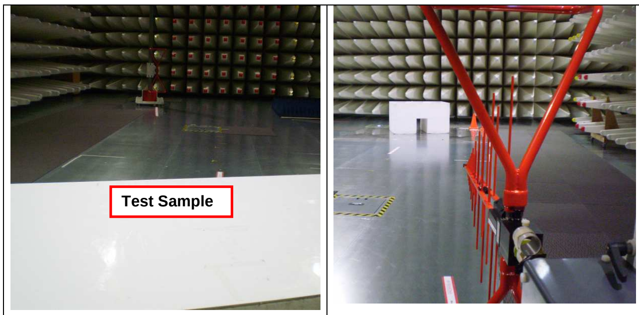
30MHz to 1000MHz – 10m Test Set-up
