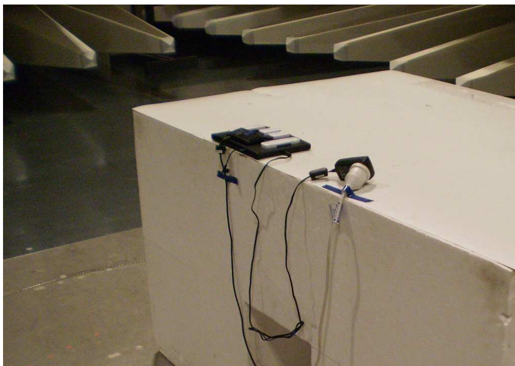
30MHz to 1000MHz – Set-up with other devices (MD-E & MD-M)
