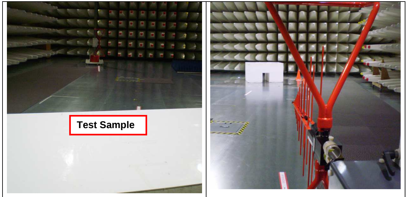
30MHz to 1000MHz – 10m Test Set-up
