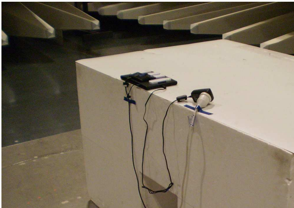
30MHz to 1000MHz – Set-up with other devices (MD-E & RFD)
