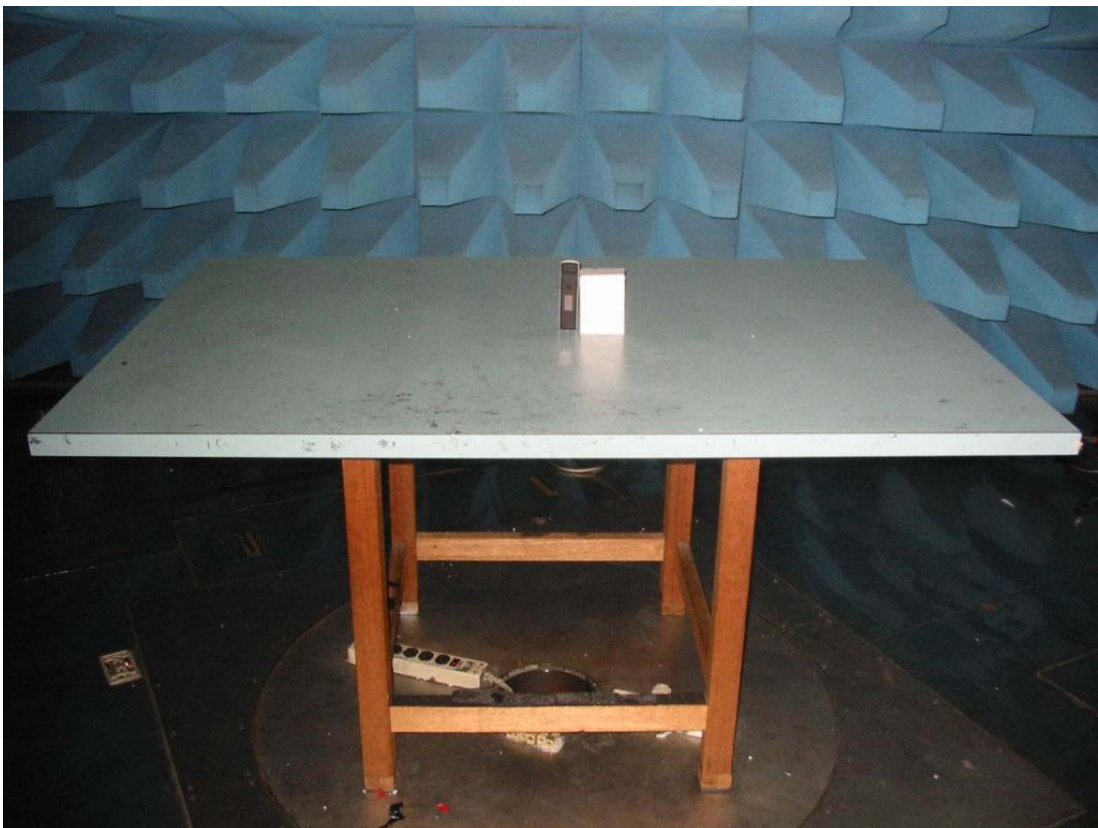
Rear View of the Test Configuration (Y-plane)
