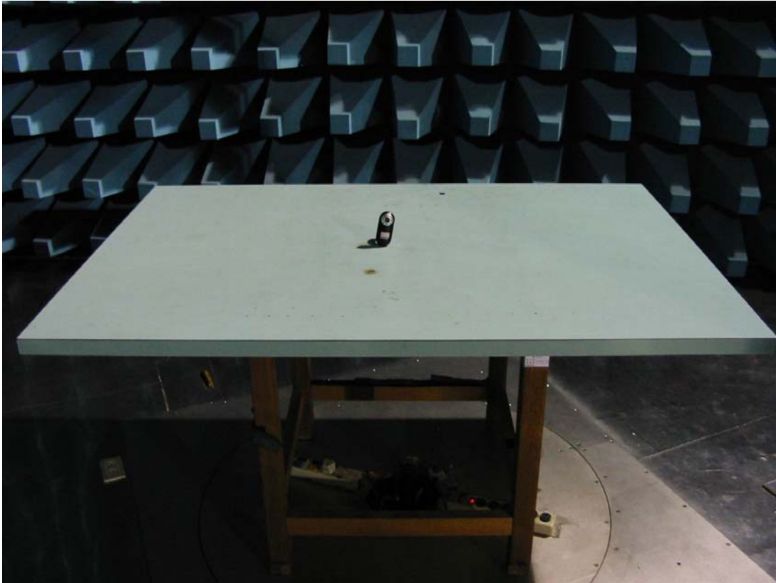
Front View of the Test Configuration (Z-plane)
