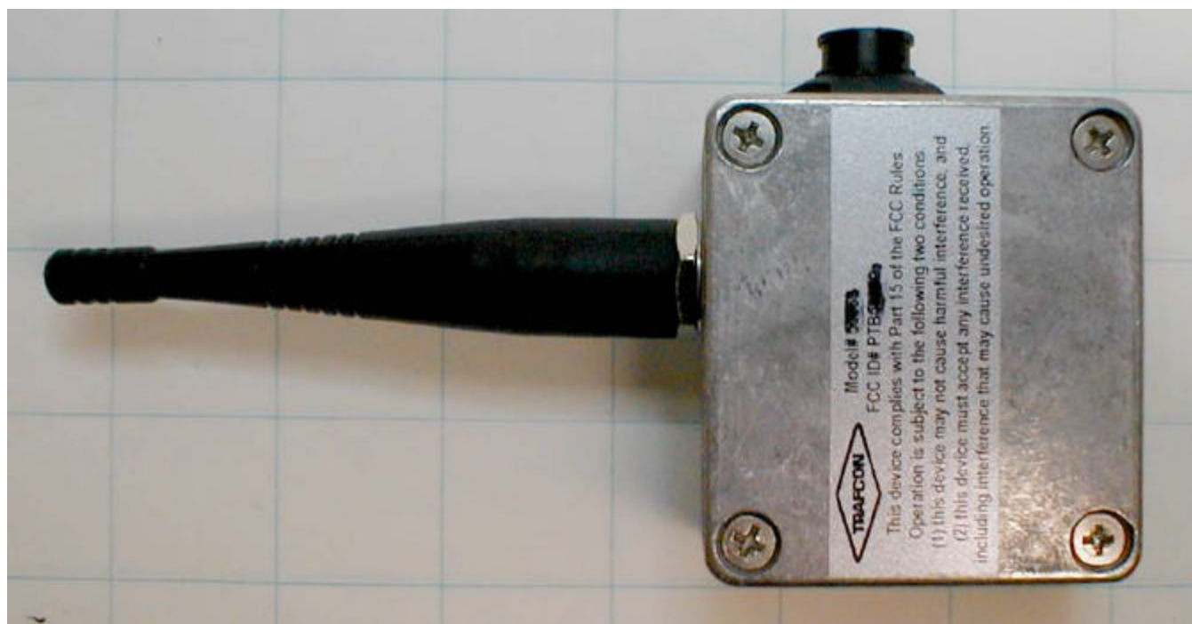
Front Panel
