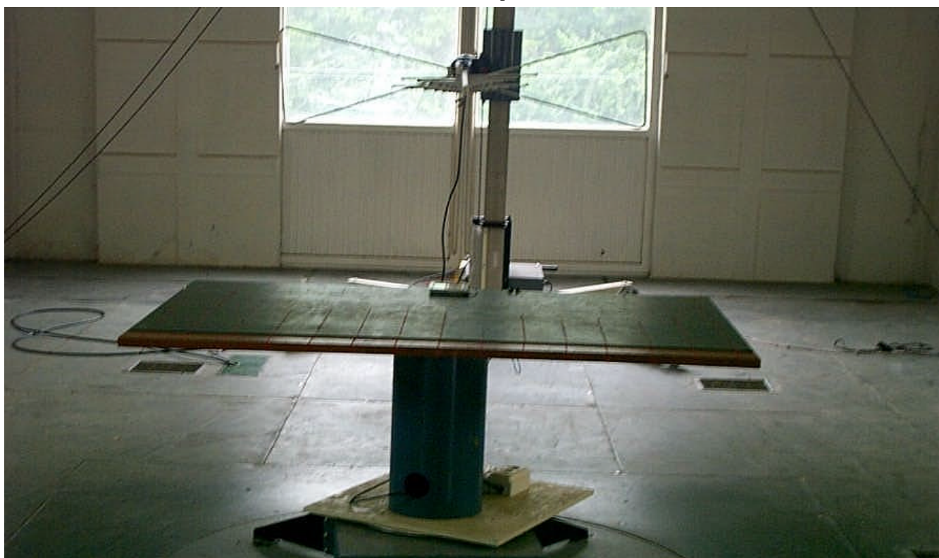
Radiated Emissions – Playback of MP3 Files
