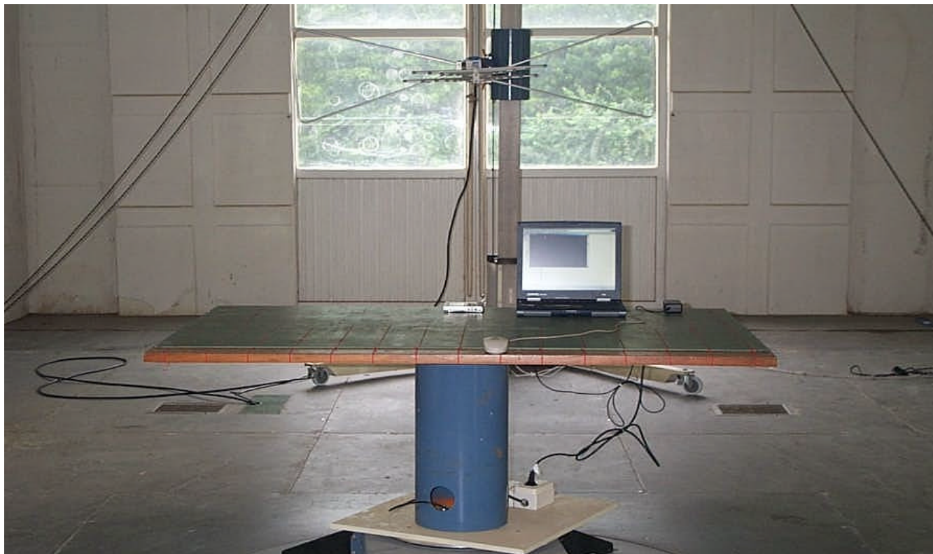
Radiated Emissions – Upload/DownLoad
