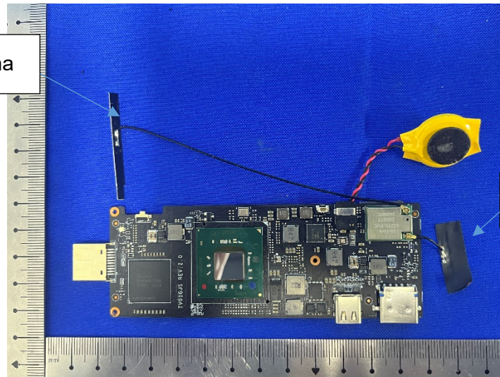
Secondary antenna
