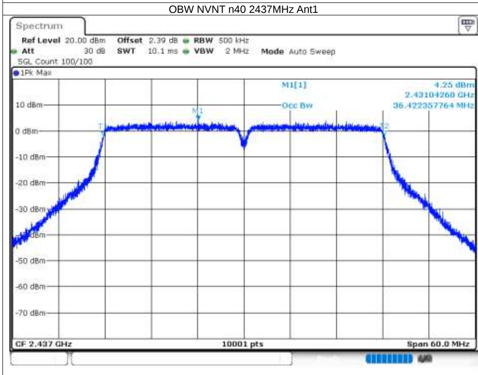
OBW NVNT n40 2437MHz Ant1
