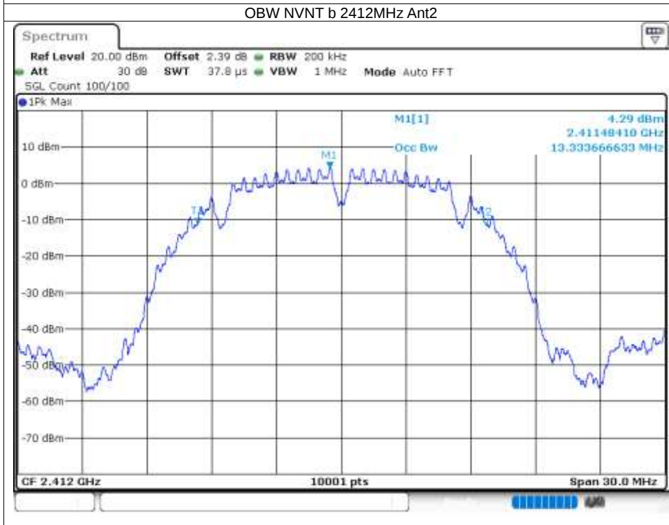
OBW NVNT b 2412MHz Ant2
