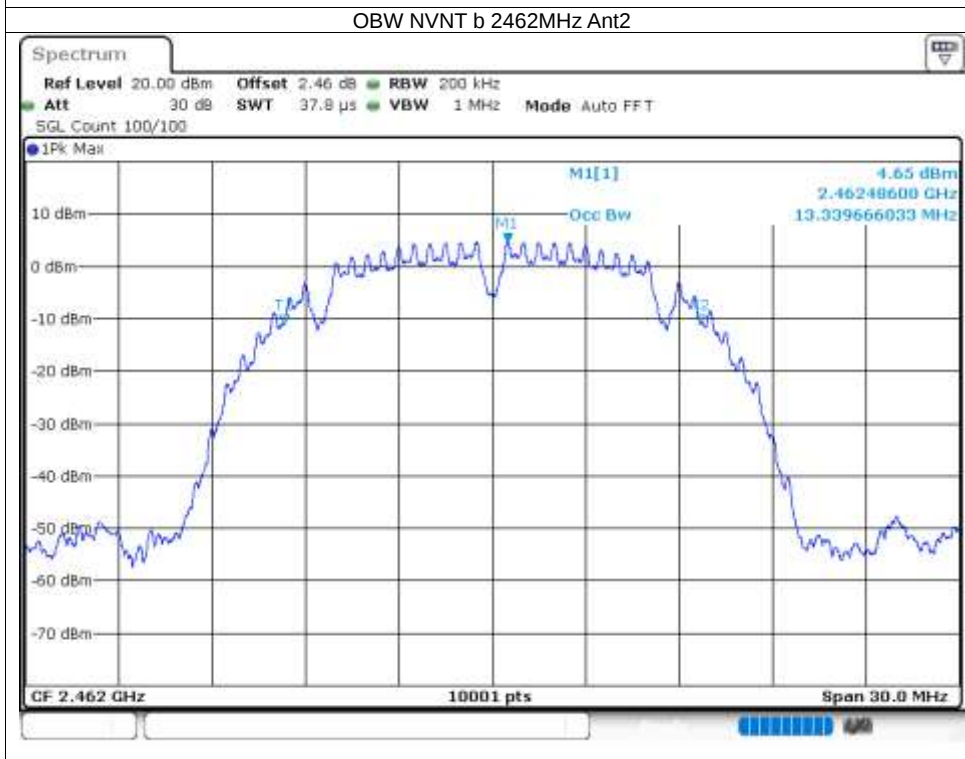
OBW NVNT b 2462MHz Ant2
