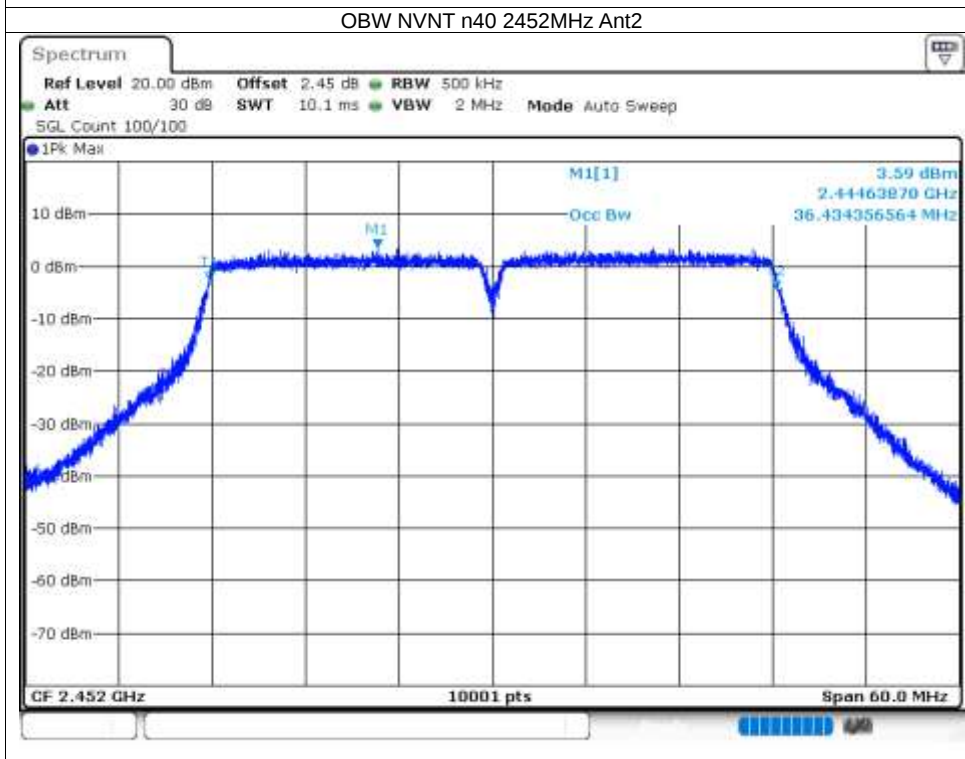
OBW NVNT n40 2452MHz Ant2
