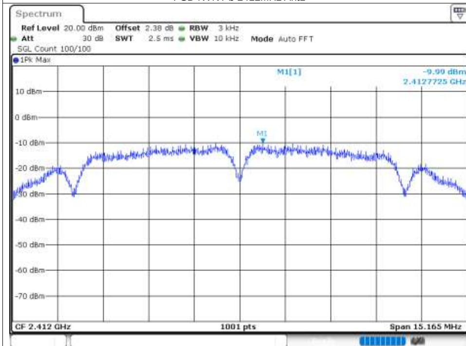
Test Graphs PSD NVNT b 2412MHz Ant1
