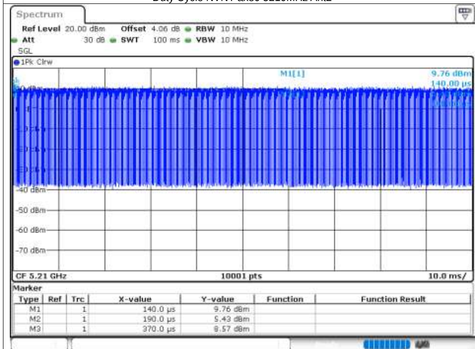
Duty Cycle NVNT ax80 5210MHz Ant2
