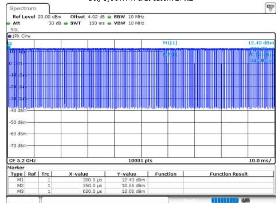
Duty Cycle NVNT ax20 5200MHz Ant1
