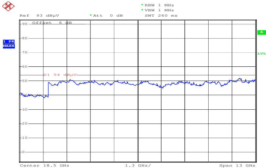
Plot 3: 12 – 25 GHz horizontal / vertical (valid for all three channels)
