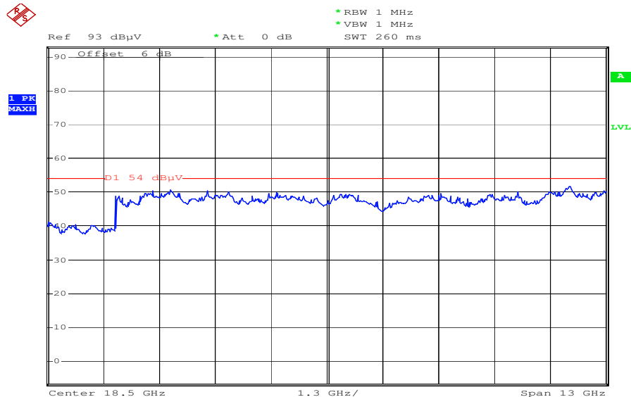
Plot 3: 12- 25 GHz (receiver)
