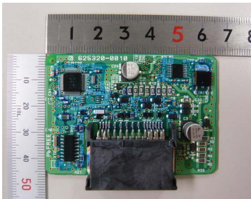
PC board (Reverse View)
