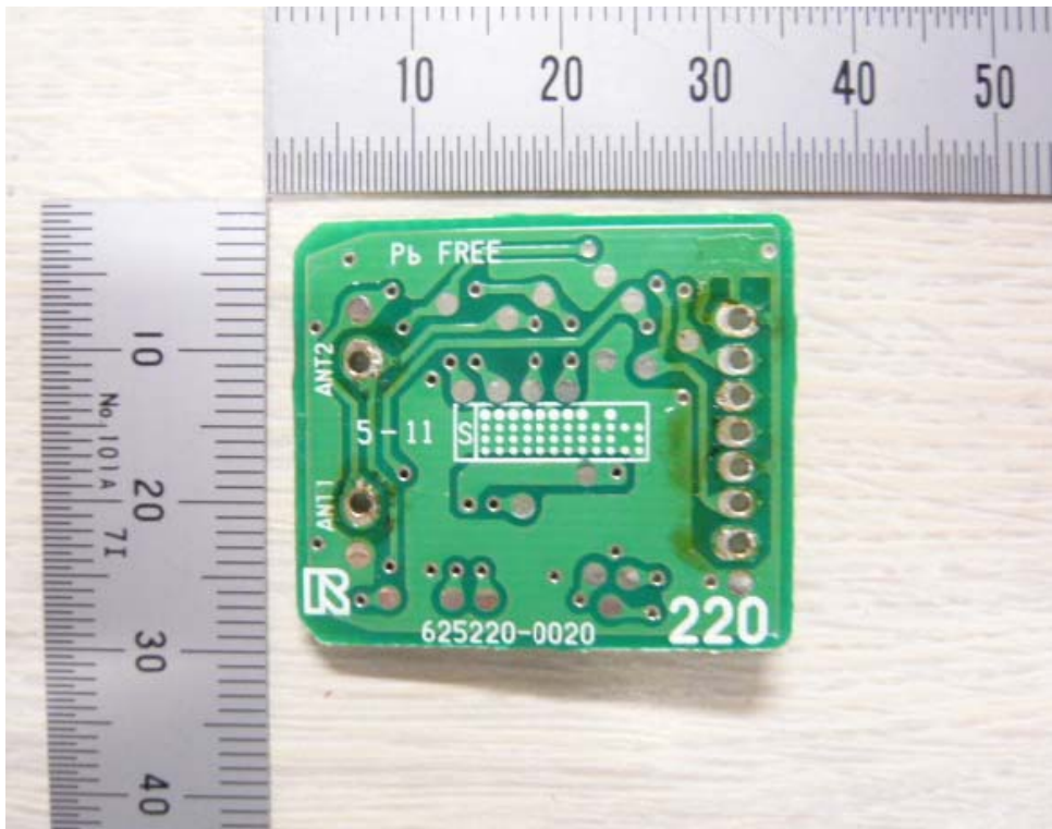
PC board (Rear View)
