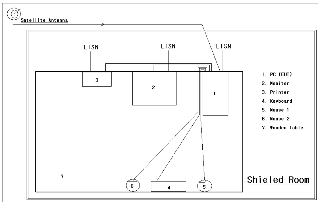
Conducted Emissions 0.15 MHz - 30 MHz
