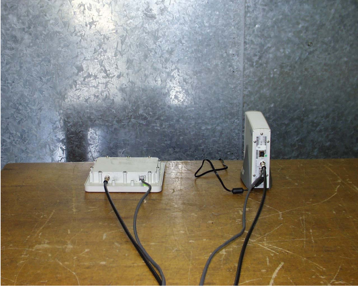
AC line conducted set-up
