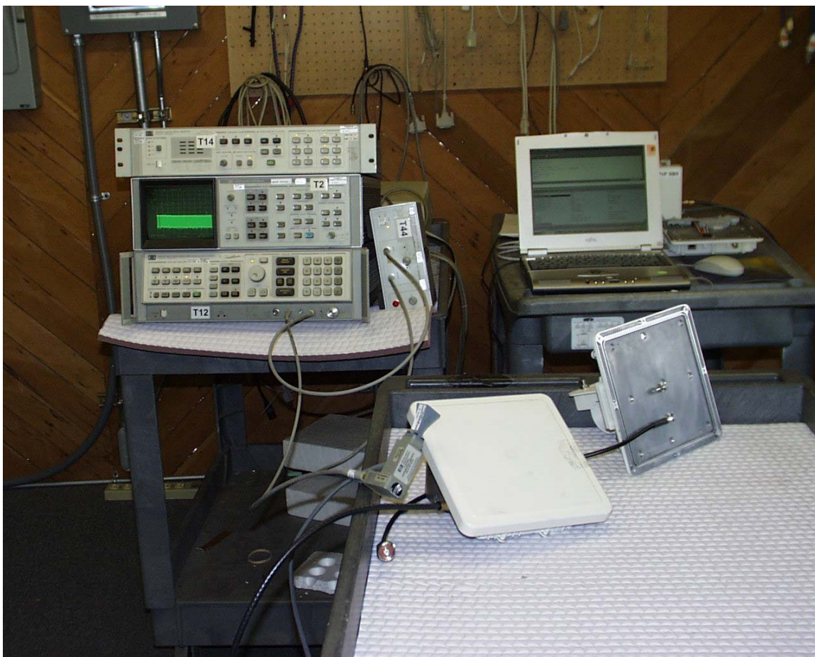
Radiated test equipment, 26 - 40 GHz
