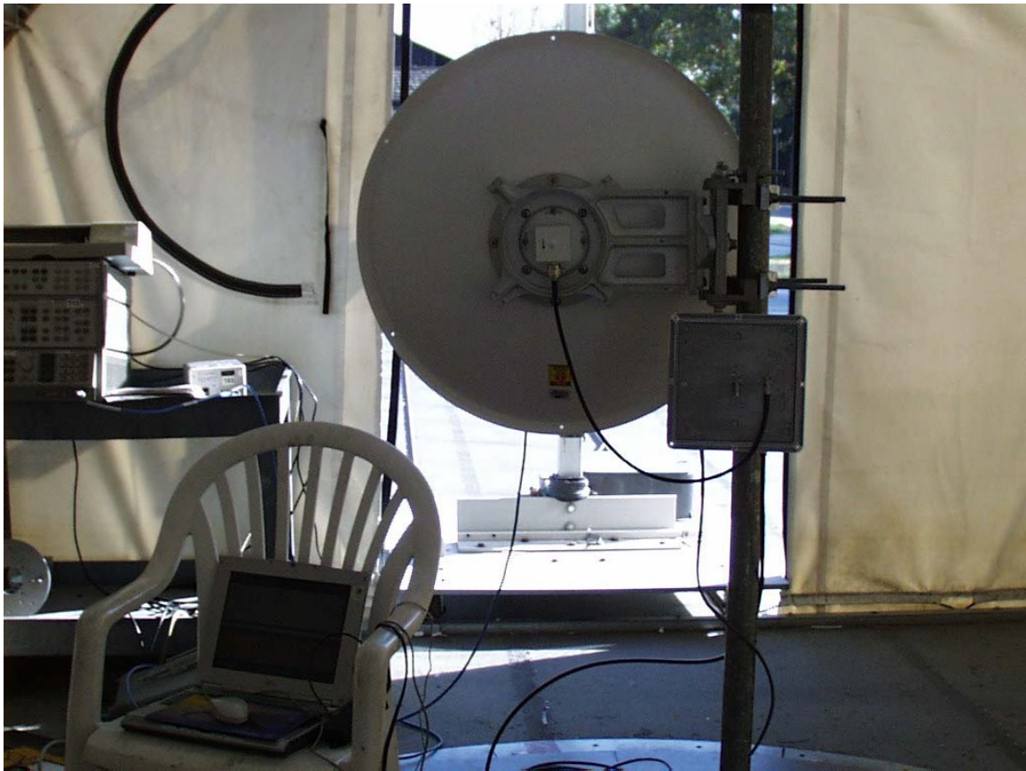
Detail, radiated dish antenna
