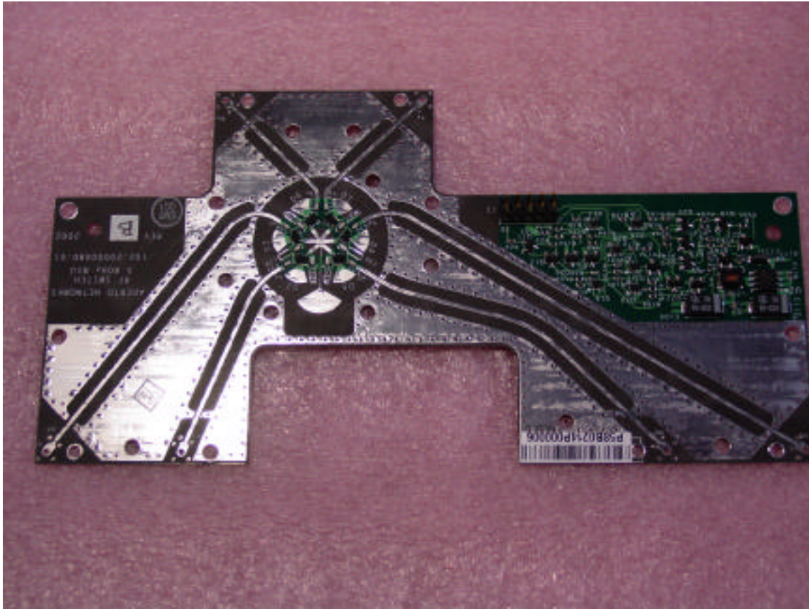
Detail 6 antenna switch, component side of board
