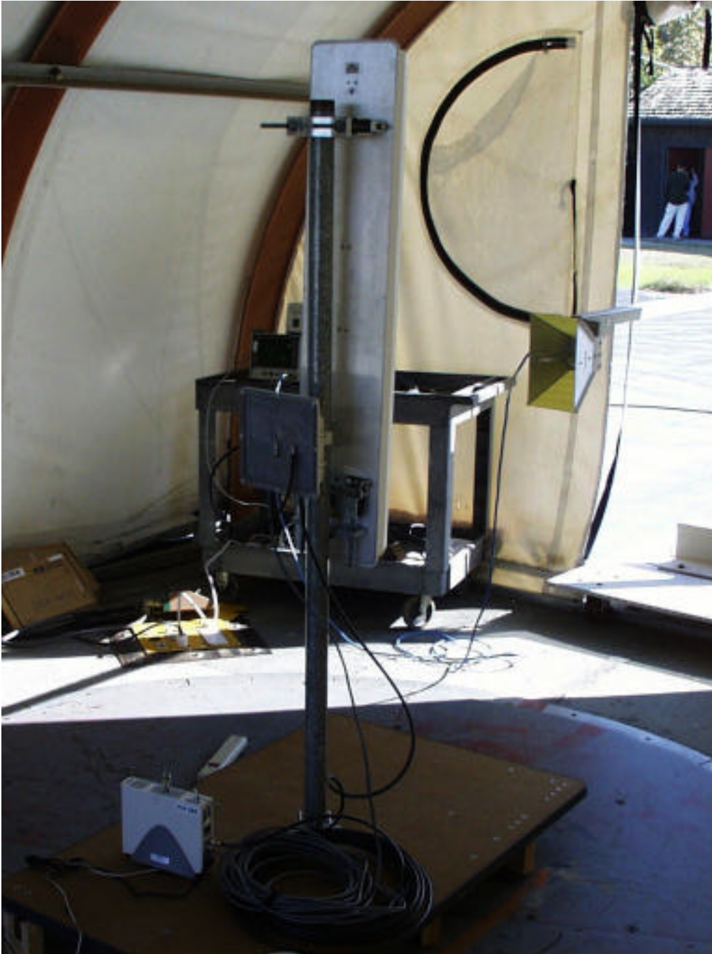
Radiated Emissions, sector antenna, rear view
