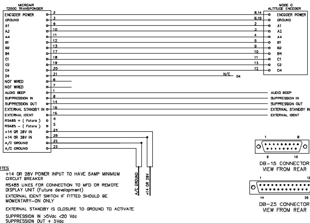
MICROAIR T2000 – WIRING DIAGRAM
