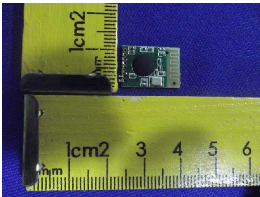
Figure 12 PCB of the EUT-Front View(wireless Module)
