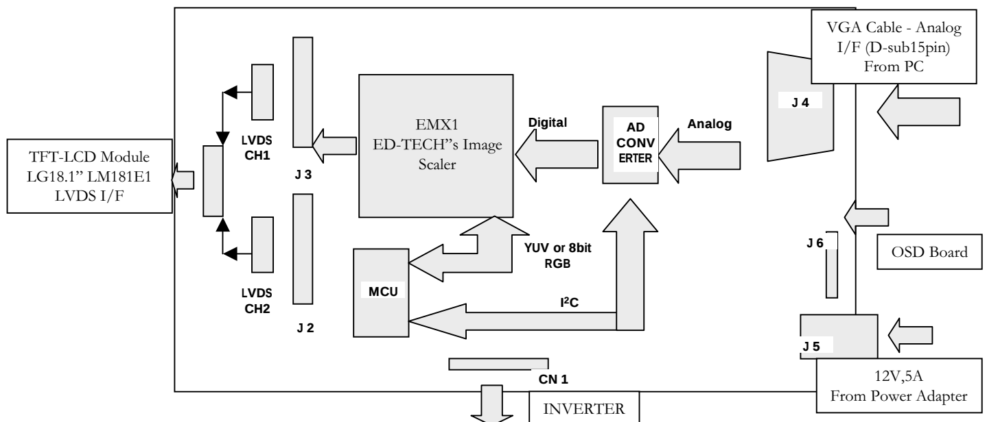
[ Fig. 2. Board Block Diagram ]
