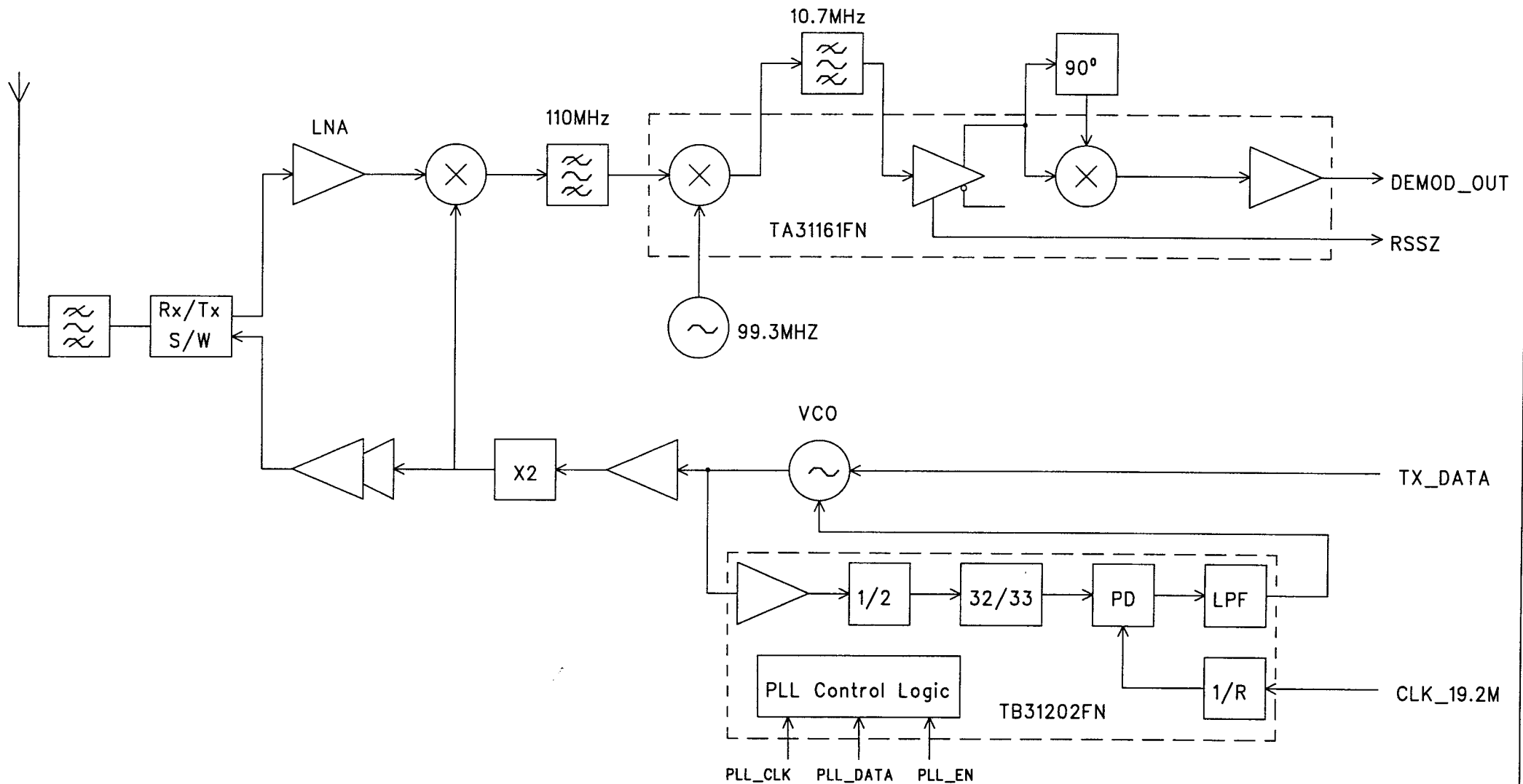
FT901 Cordless Phone RF Module Block Diagram
