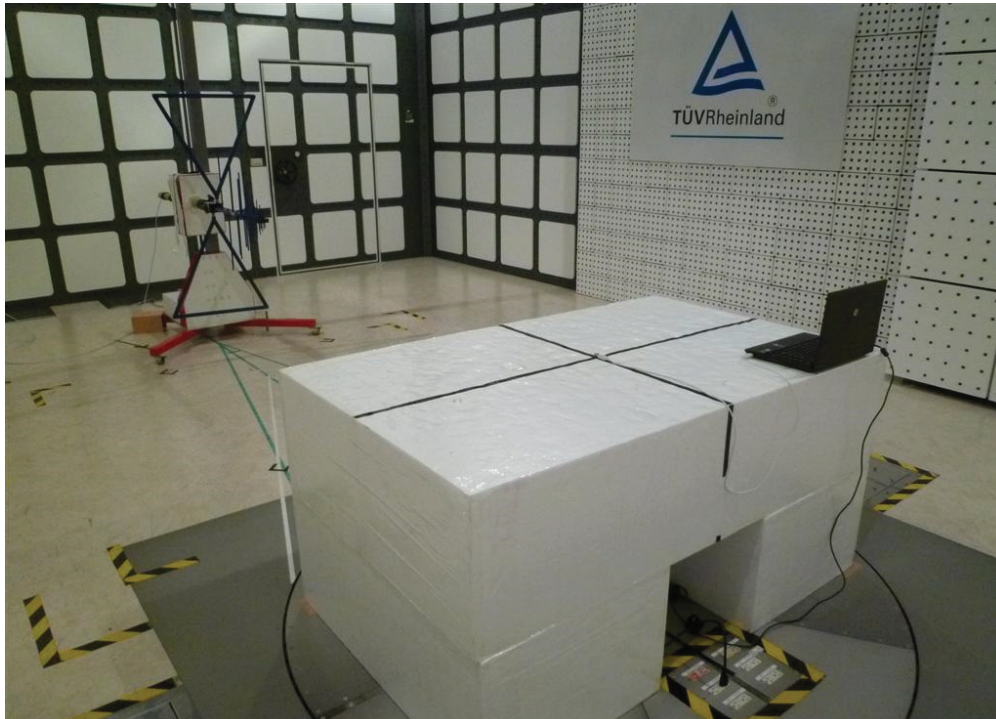
Photograph 3: Set-up for Spurious Emissions (Back View 2 TX)
