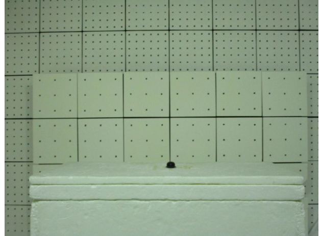
Part_15.249_2.4G_Radiated_Setup
