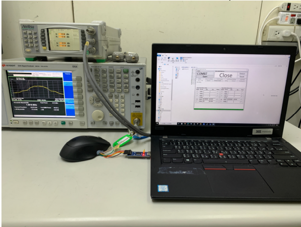
Part_15.249_2.4G_Conducted_Setup
