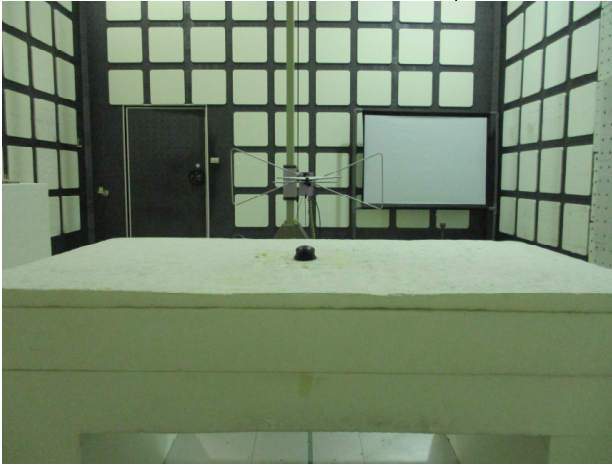
Part_15.249_2.4G_Radiated_Setup
