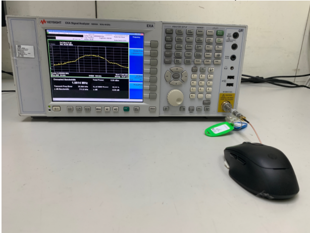
Part_15.249_2.4G_Conducted_Setup
