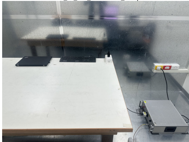
Part_15_249_Conduction_Setup
