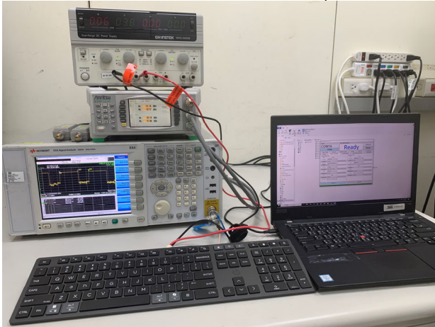
Part_15_249_Conducted_Setup
