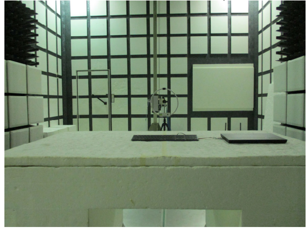
Part_15_249_Radiated_Setup
