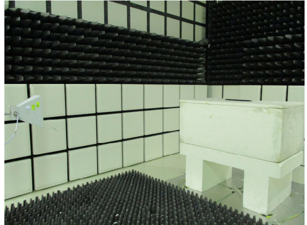
Part_15_249_Radiated_Setup
