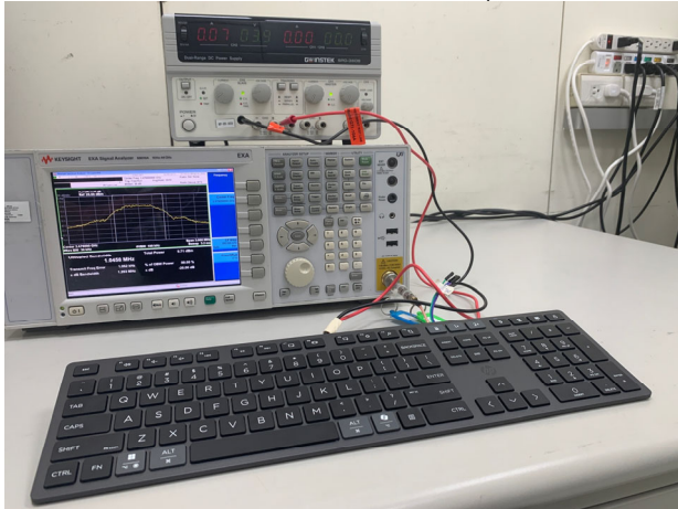
Part_15_249_Conducted_Setup
