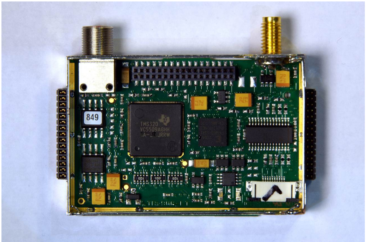
Figure 4: DSP Board – Top View With Shielding
