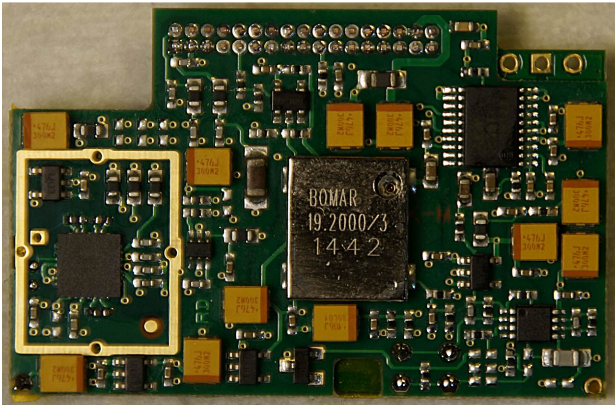
Figure 2: Audio Board – Top View Without Shielding
