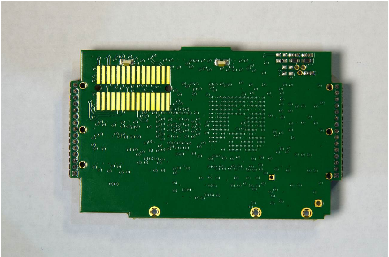
Figure 7: DSP Board – Bottom View Without Shielding
