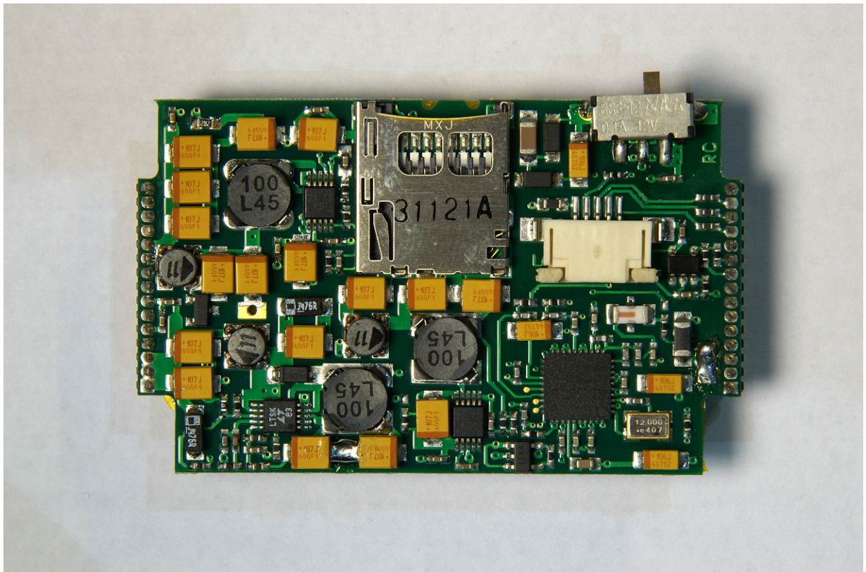
Figure 8: Power Supply Board – Top View
