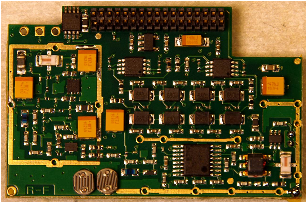
Figure 11: RF Board – Top View Without Shielding
