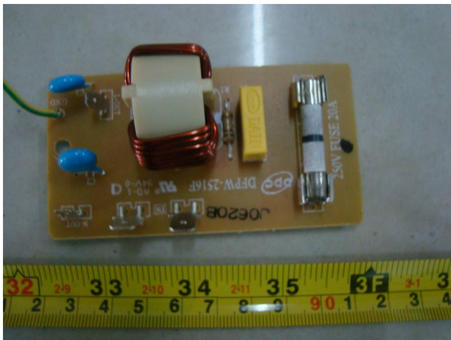
EUT – EMI Filter Board Top Components View
