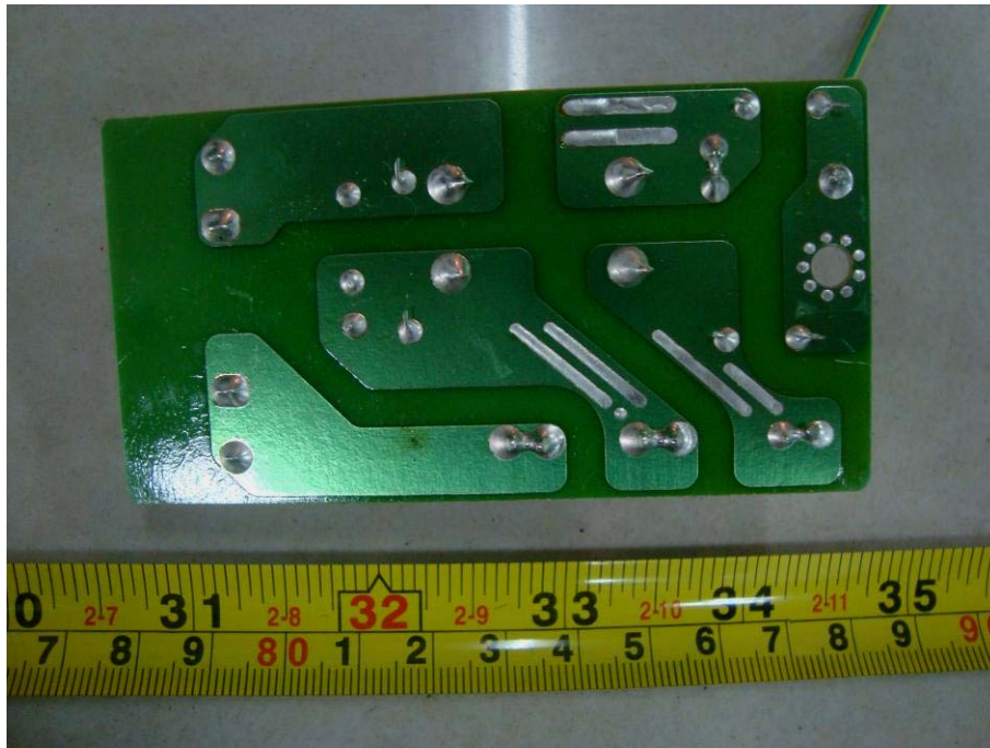
EUT – EMI Filter Board Bottom Circuit View
