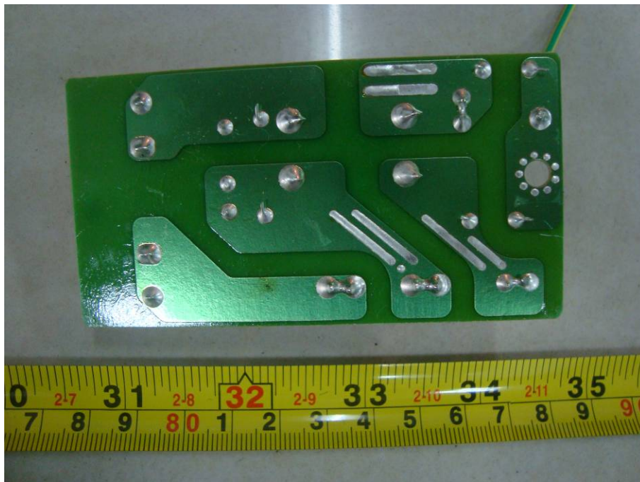
EUT – EMI Filter Board Bottom View
