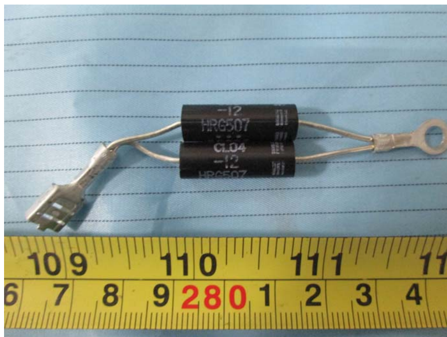
EUT – HRG507 View
