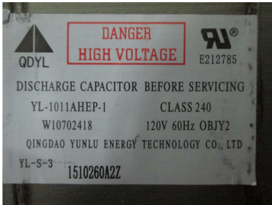
EUT – Discharge Capacitor Label View
