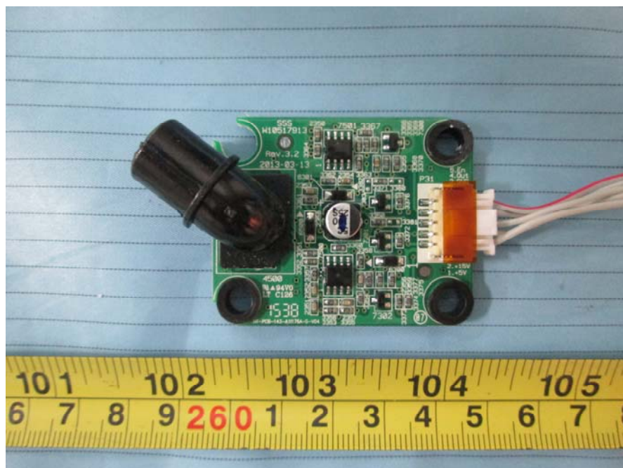
EUT – Main Board 3 Top View 1
