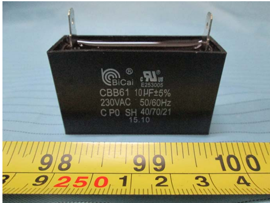
EUT – CBB61 View
