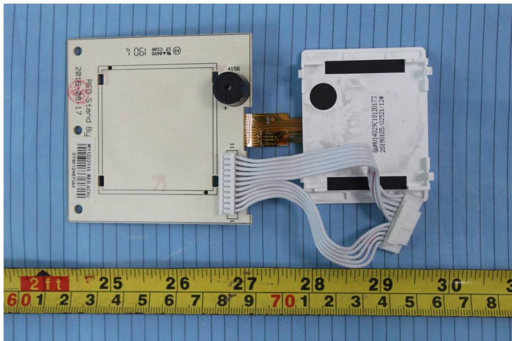
EUT – LCD Cover off View
