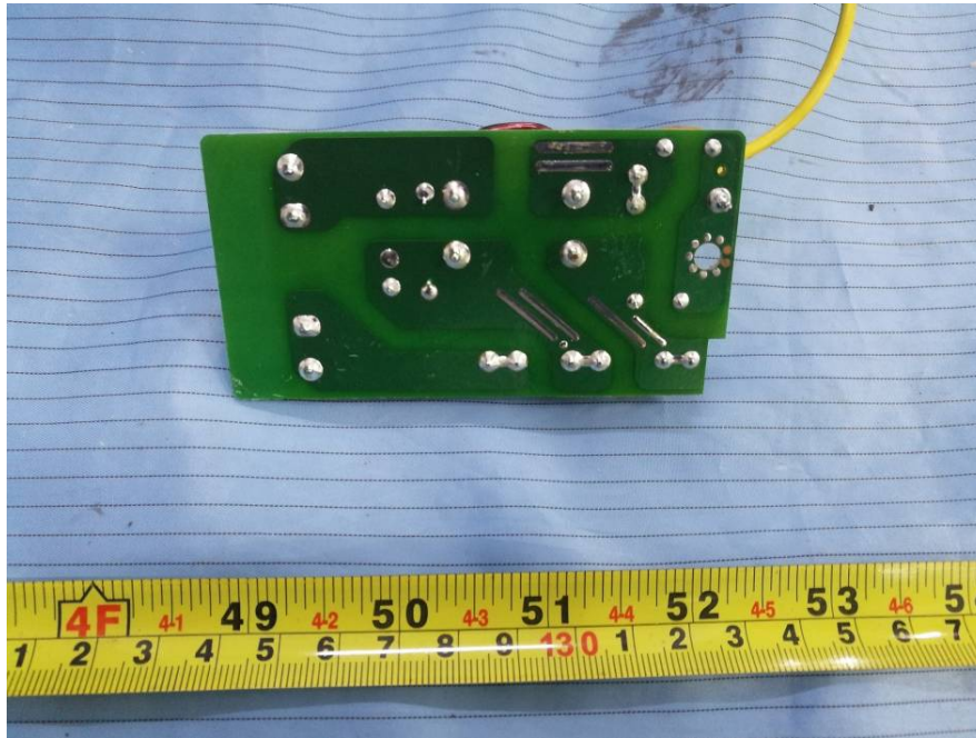
EUT – Filter Circuit Board Bottom View
