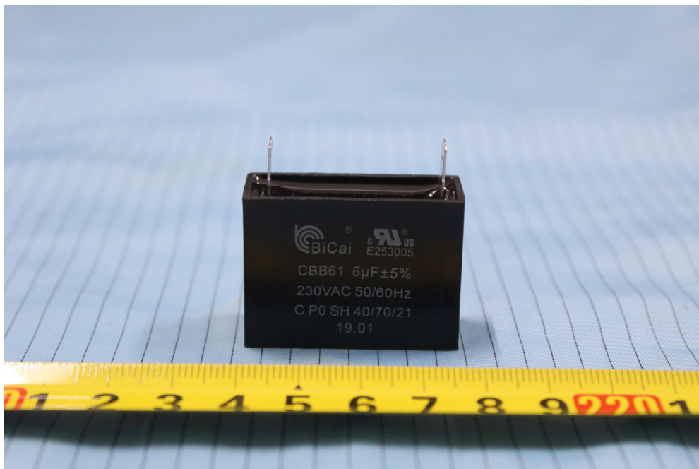
EUT – Capacitor View
