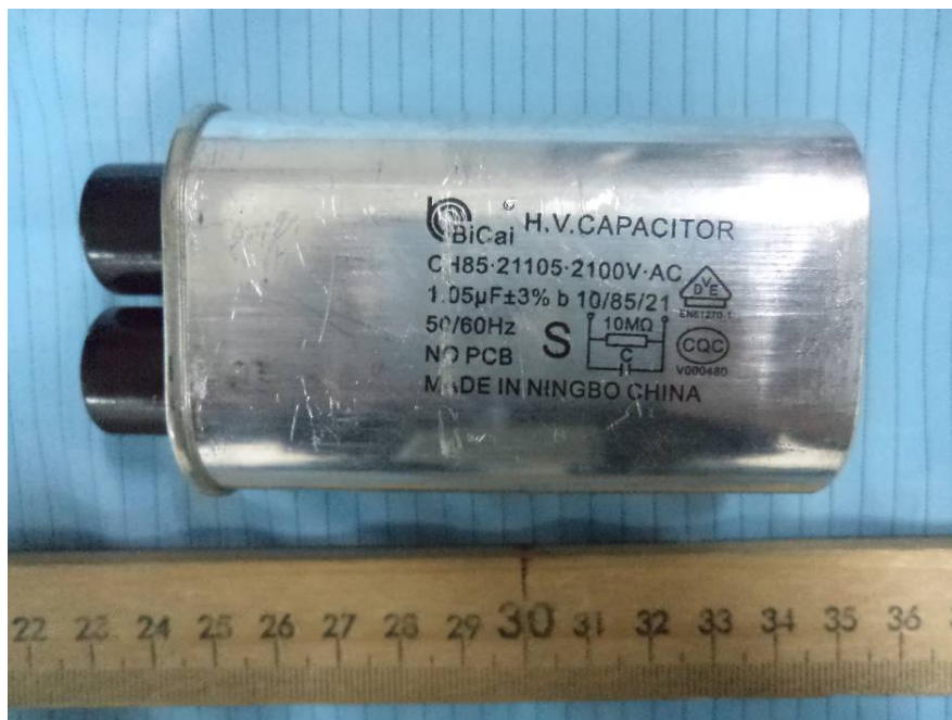
EUT – H.V. Capacitor View
