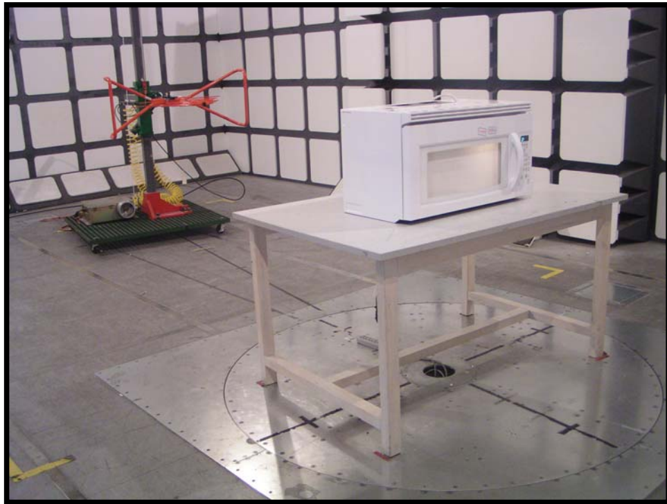
Radiated Emissions-Front View (30 MHz-1000 MHz)
