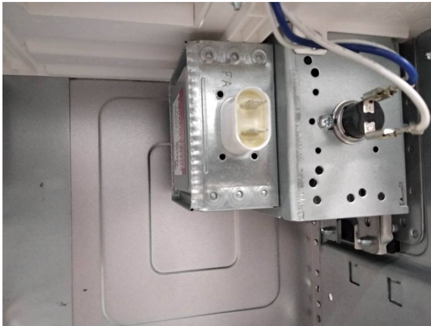
EUT – Magnetron View
