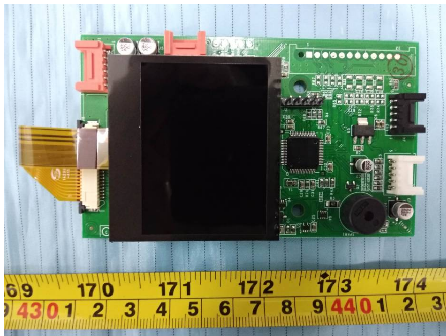
EUT – LCD Board Front View
