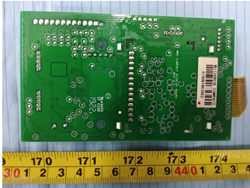
EUT – LCD Board Rear View
