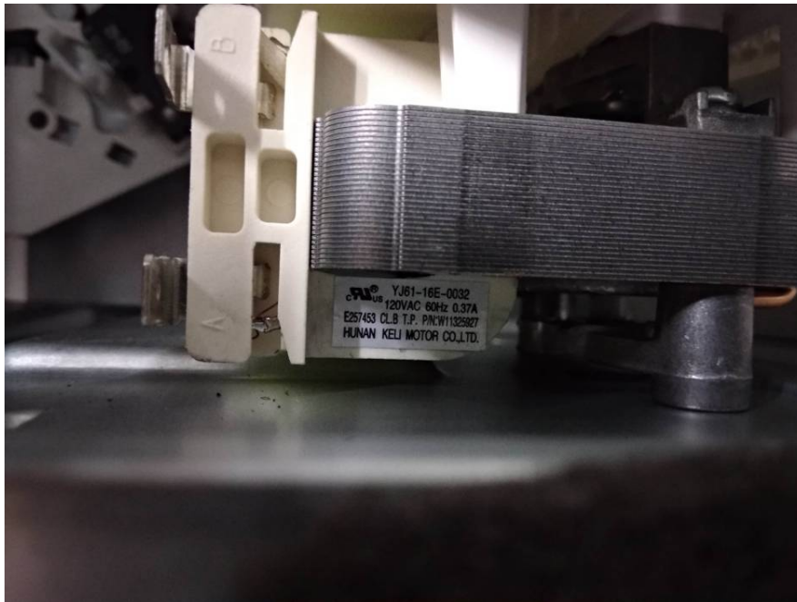
EUT – Motor 2 Label View
