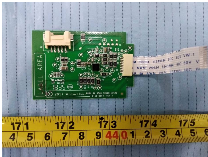
EUT – Touch Board Front View
