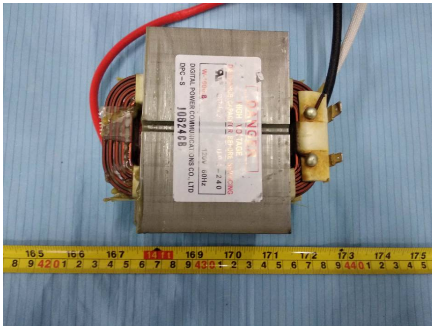
EUT – Transformer Front View
