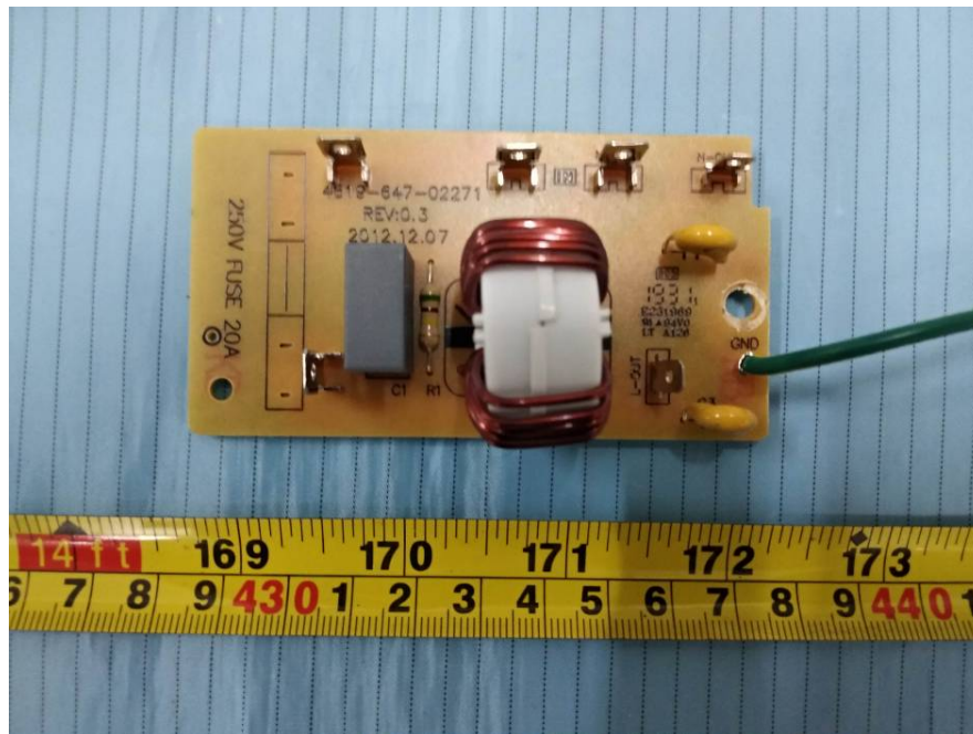
EUT – Power Supply Board Front View
