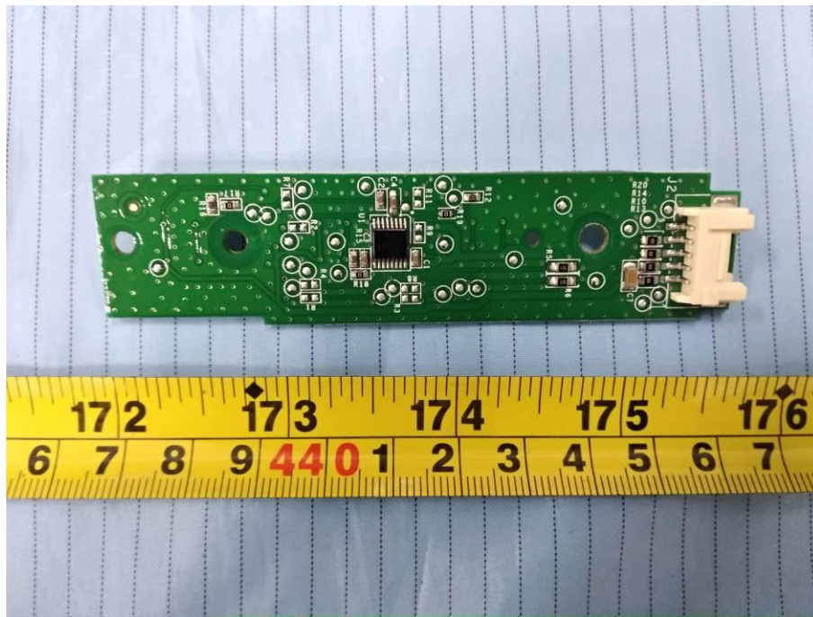
EUT – Keypad Board Bottom View
