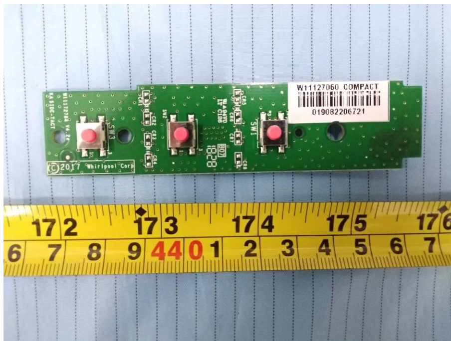
EUT –Keypad Board Top View
