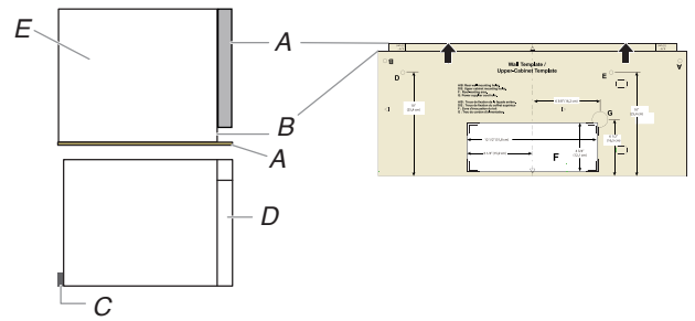
A. Front Edge of Cardboard Plate & Upper Cabinet Door B. Upper Cabinet & Cardboard Plate 0.75" (1.9 cm) Line C. Mounting plate D. Microwave oven door E. Cabinet
