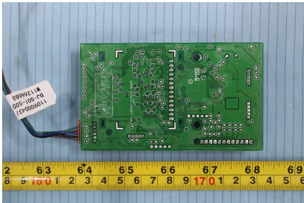
EUT –LED Display Board Bottom View
