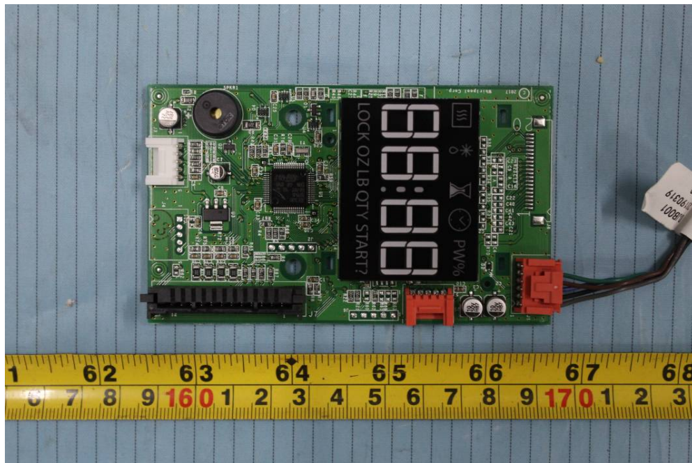
EUT – LED Display Board Top View
