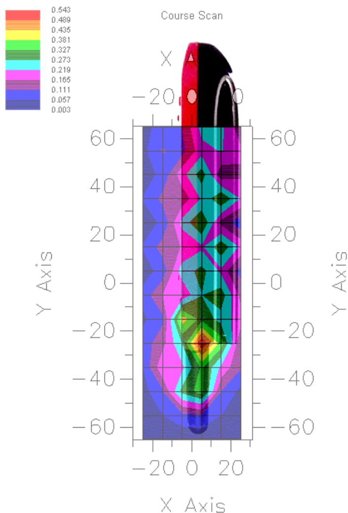
GRAPH 7 RIGHT SIDE Distance: 0 mm High Channel – 821 MHz
