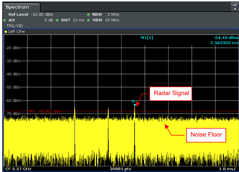
Single Burst of Radar Signal 5
