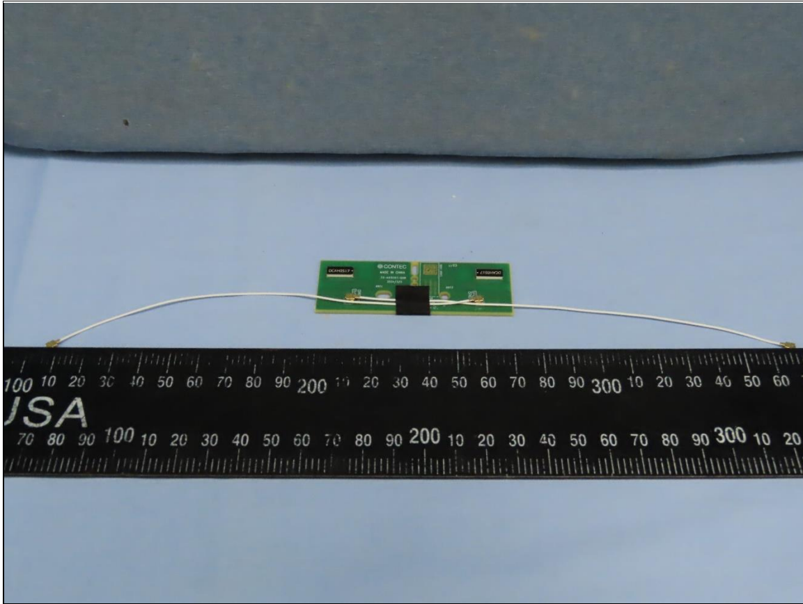
ANT Set 2 (Brand: CIROCOMM / Model: DCAH0S17)
