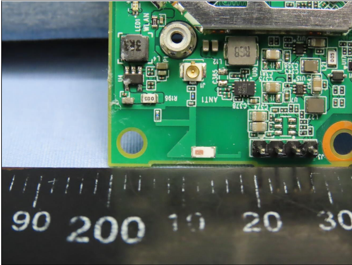
ANT Set 1 (Brand: Johanson / Model: 2450AD18A6050)
