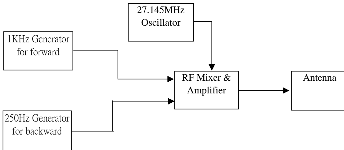
Wiggle RC Car 27.145MHz Tx Block Diagram
