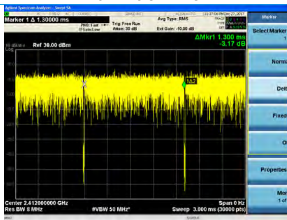
MCS0 Off Time
