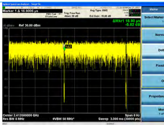
6 MBPS Off Time
