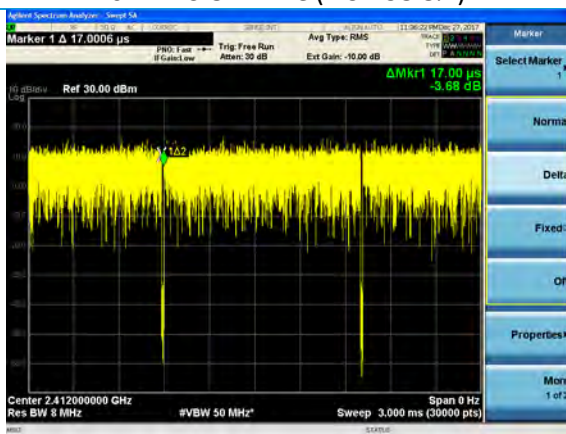
MCS0 On Time (DC = 98.7%)
