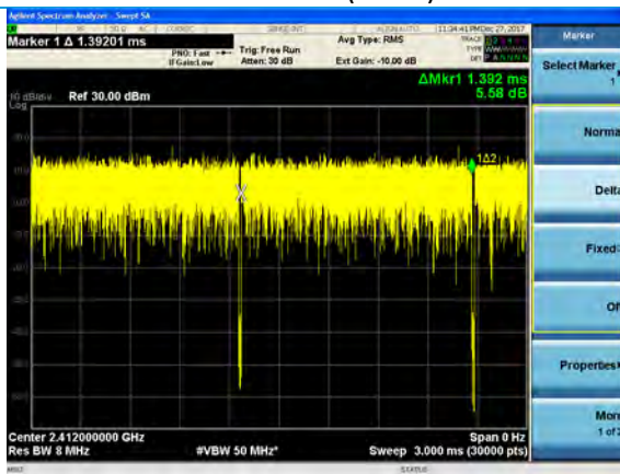
6 MBPS On Time (DC = 98.8%)
