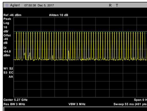
Plot 9. Radar Waveform Calibration, 5270 MHz, Type 1, 40 MHz
