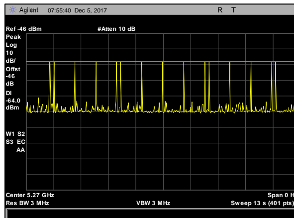
Plot 13. Radar Waveform Calibration, 5270 MHz, Type 5, 40 MHz
