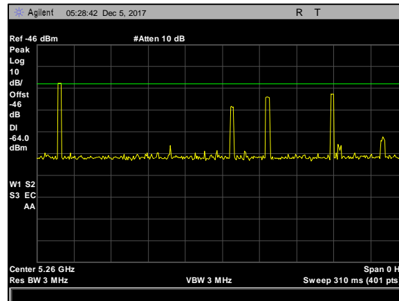
Plot 7. Radar Waveform Calibration, 5260 MHz, Type 6, 20 MHz
