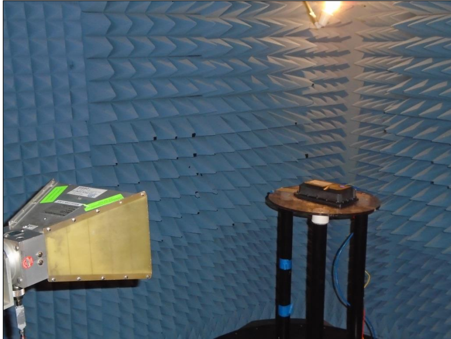
Photograph 1. Spurious Radiated Emissions, above 1 GHz Test setup (WiFi)
