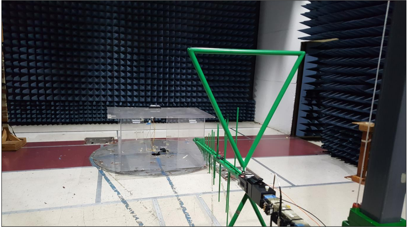
Photograph 3. Radiated Spurious Emissions, 30 MHz – 1 GHz, Test Setup (BLE)
