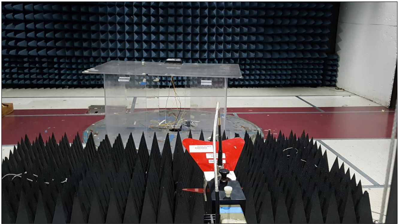
Photograph 4. Radiated Spurious Emissions, 1 – 18 GHz, Test Setup (BLE)
