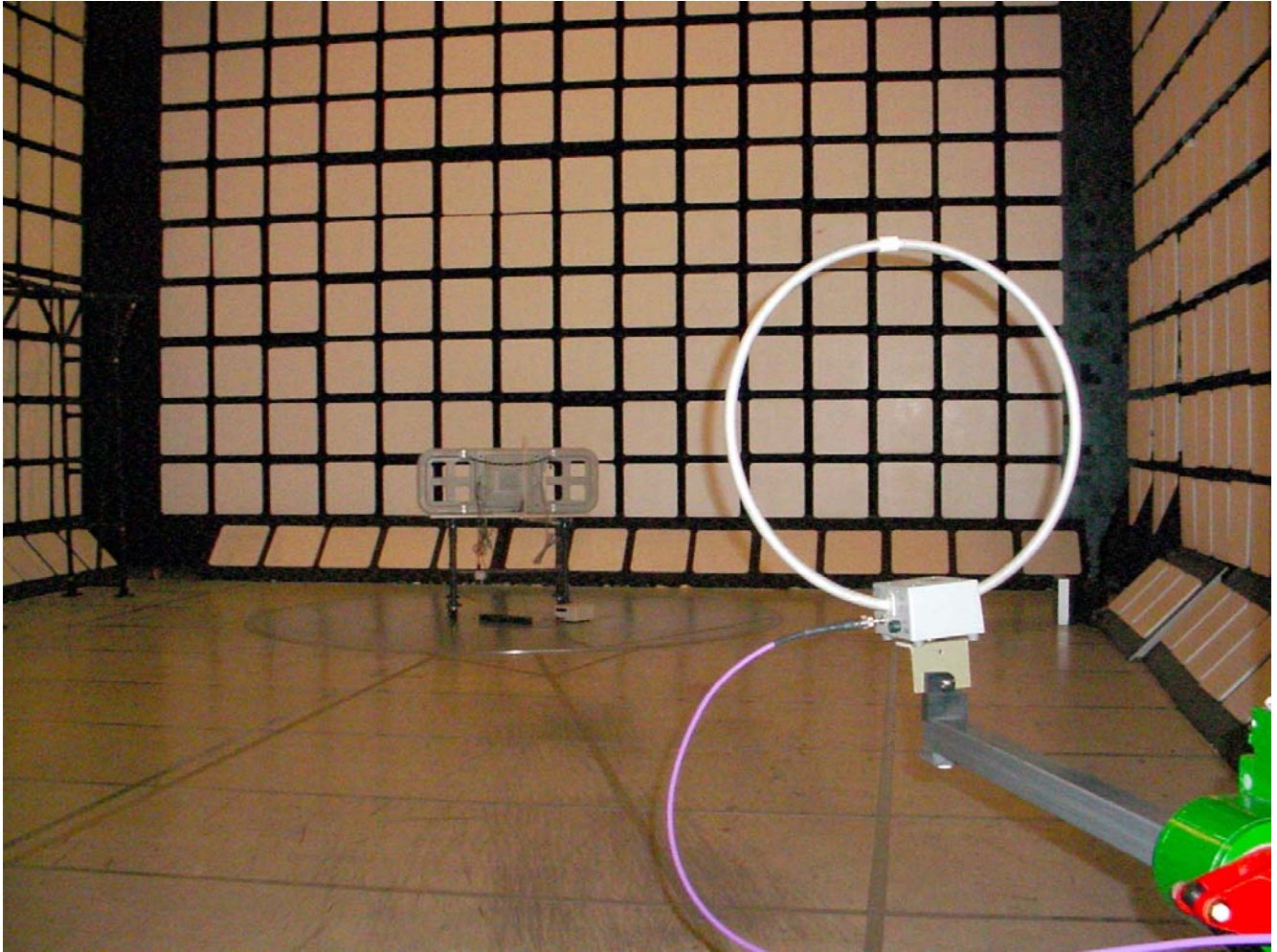
Radiated Emissions at 10m Distance
