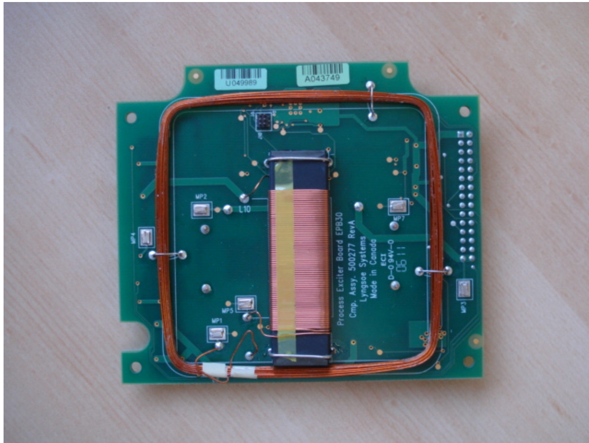
Top (daughterboard)
