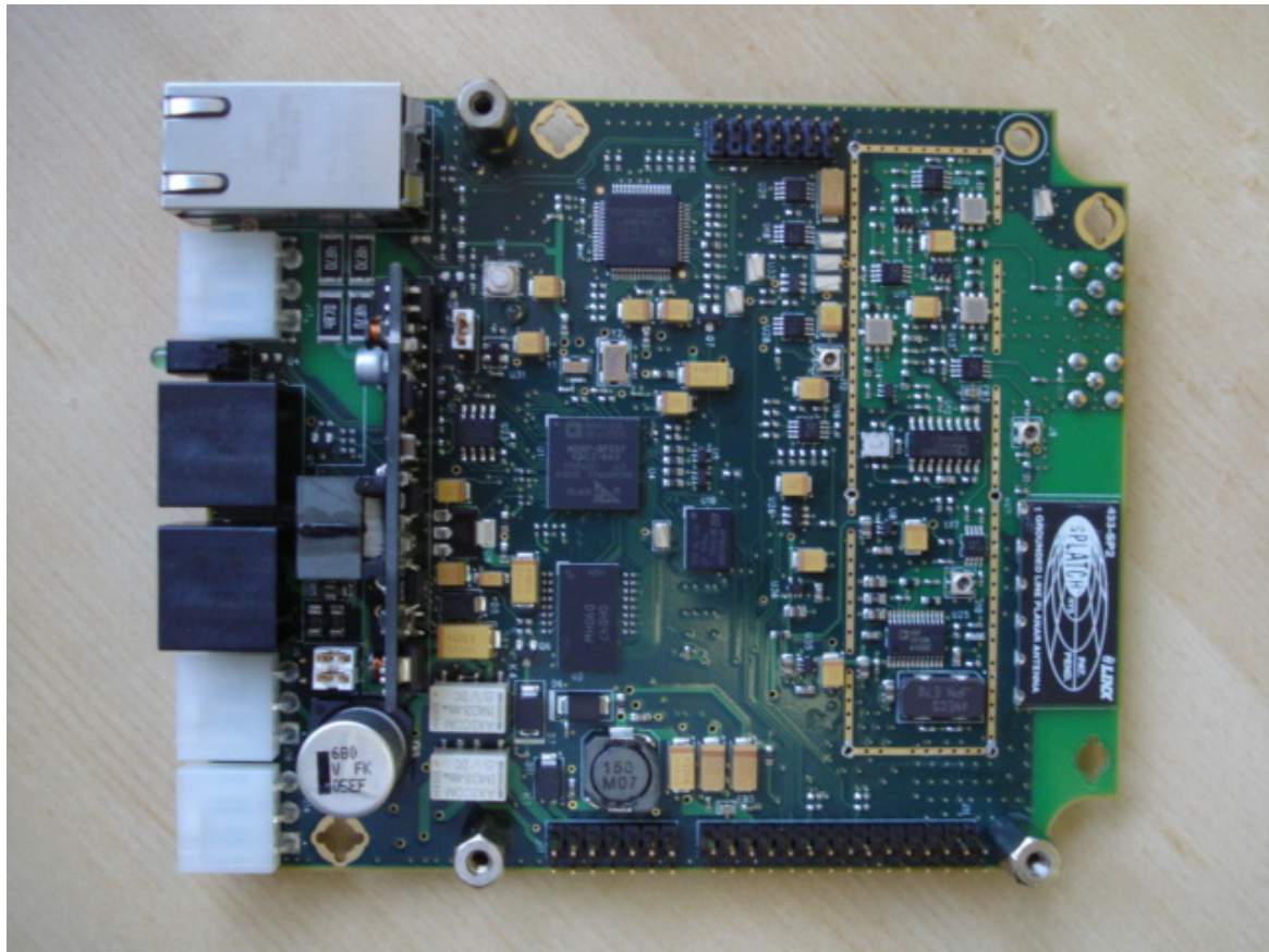
Top (master board with shield removed)
