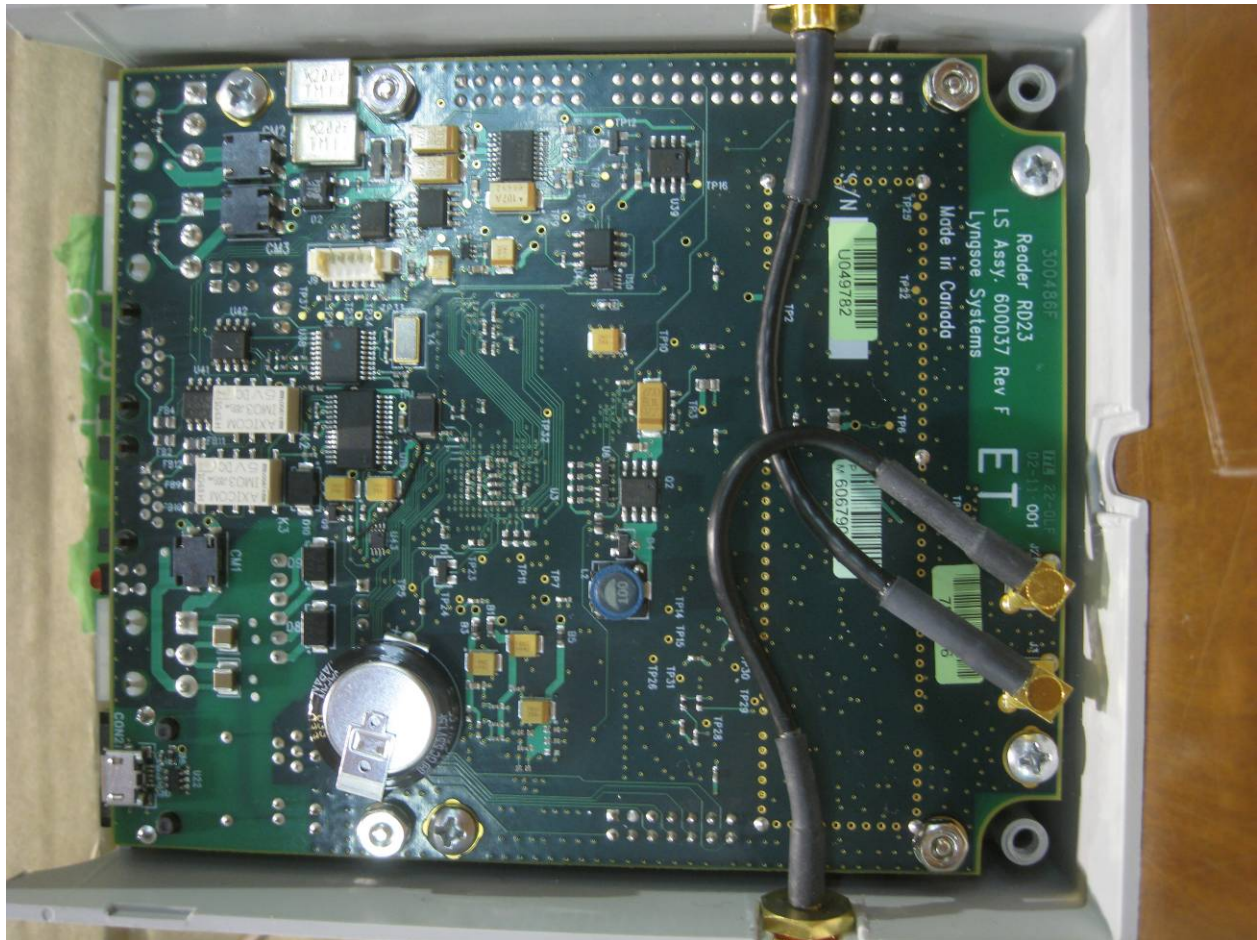
Bottom (master board)
