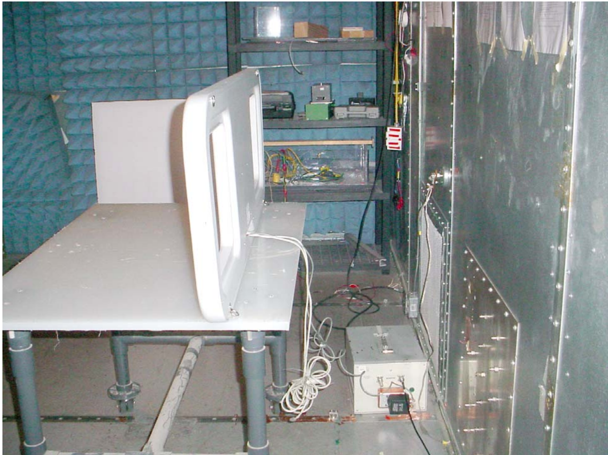
Powerline Conducted Emissions (side view)
