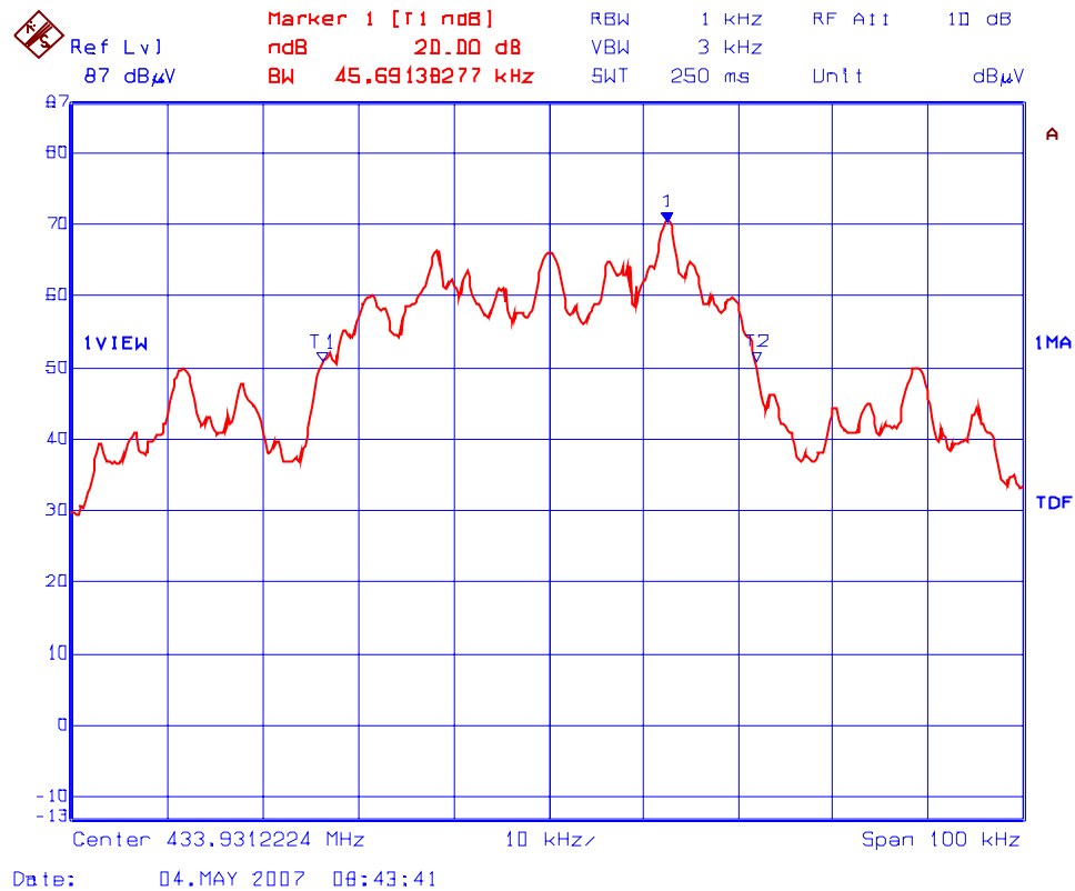
Plot 5.7.4.2: 20 dB Bandwidth (Beacon Mode) Fc: 433.92 MHz
