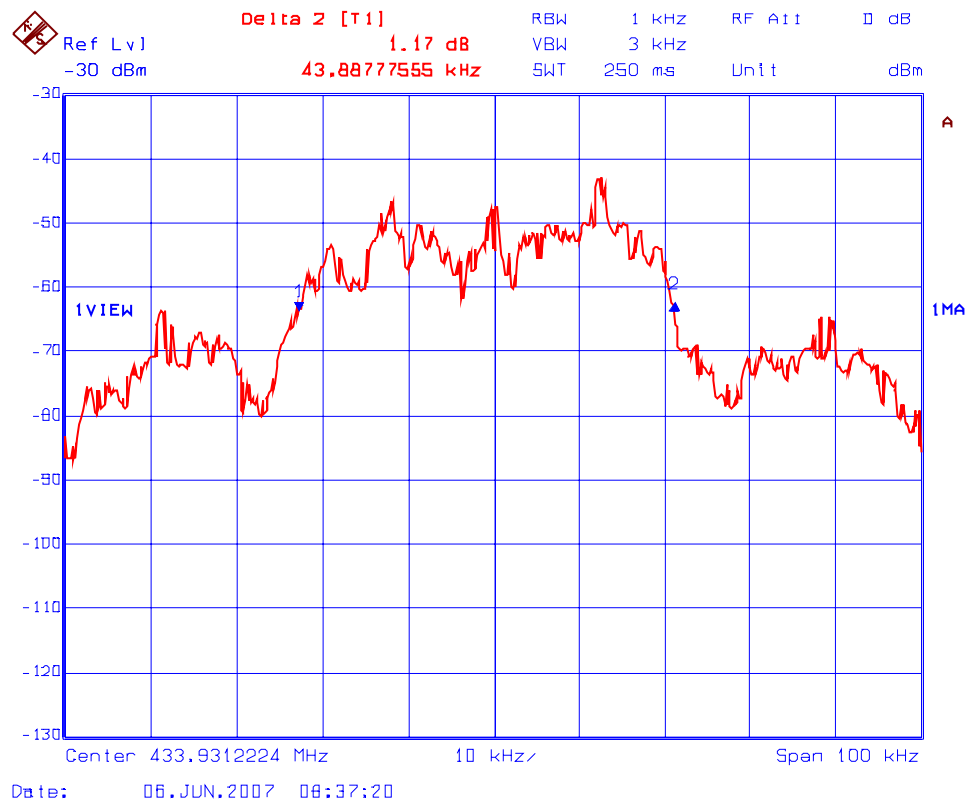
Plot 5.7.4.1: 20 dB Bandwidth (Excitation Mode) Fc: 433.92 MHz
